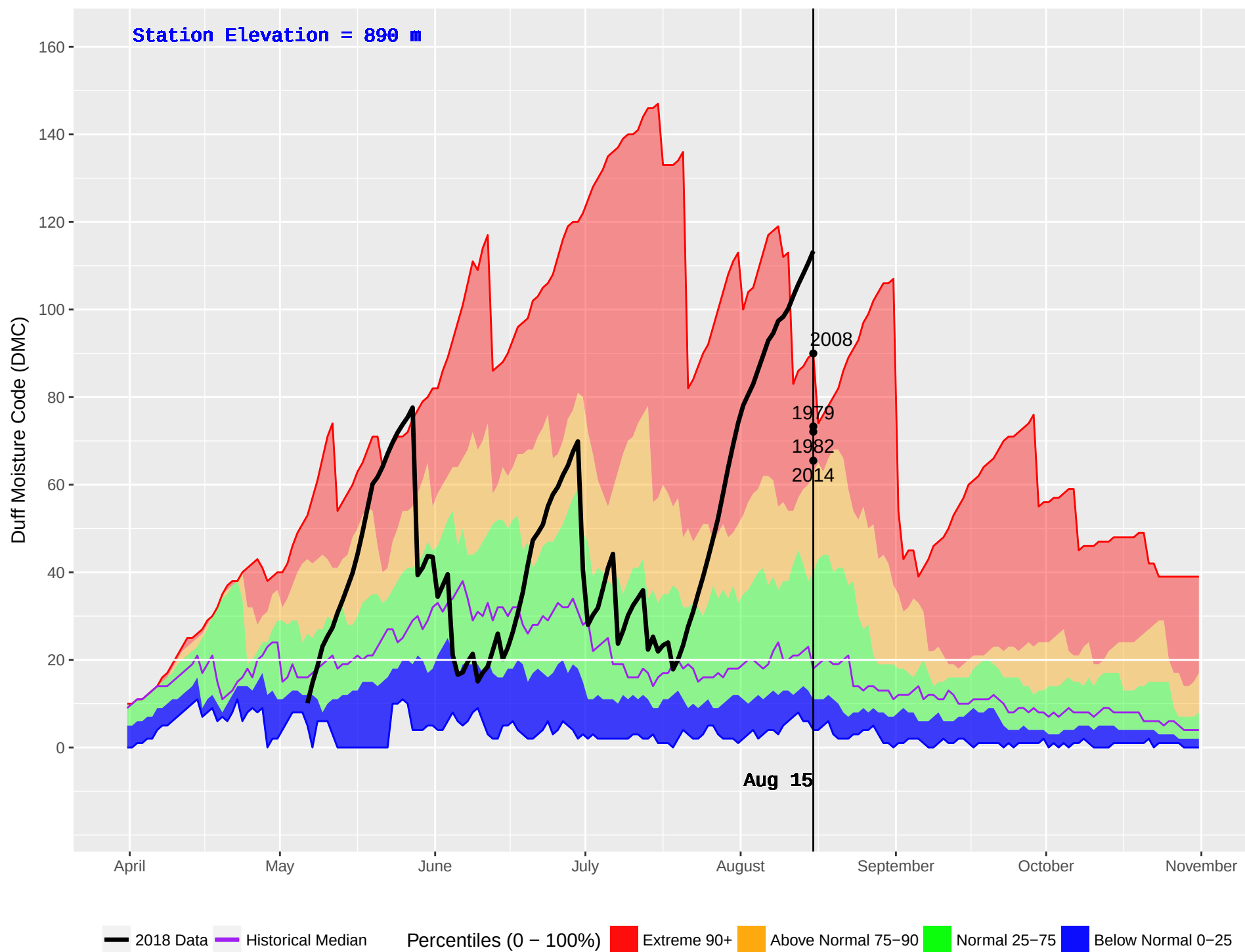
ISKUT (112) : Historical (1979–2016) and Current (2018) Daily Duff Moisture Code (DMC)
