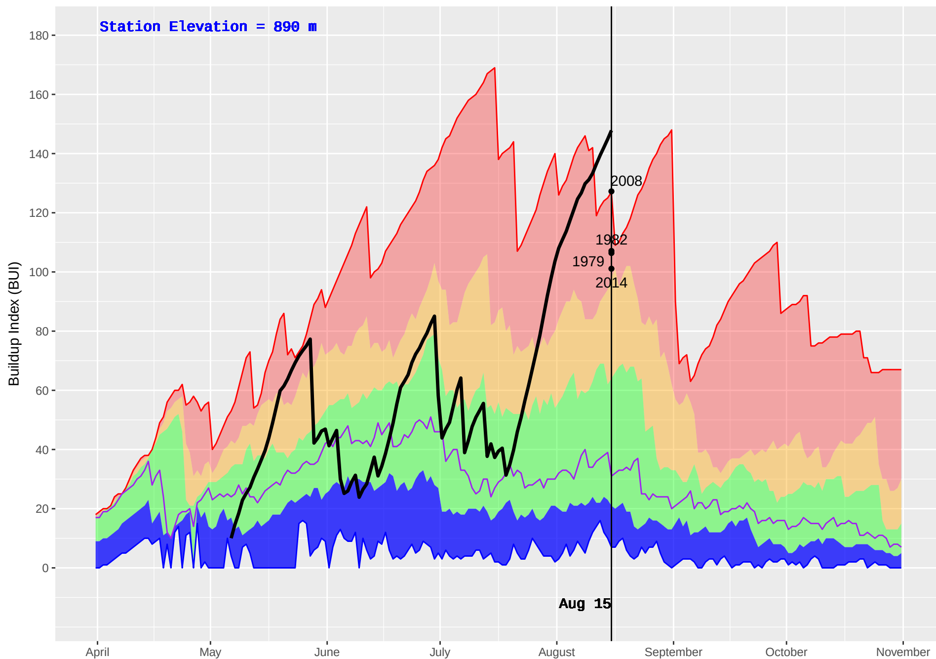
ISKUT (112) : Historical (1979–2016) and Current (2018) Daily Buildup Index (BUI)
