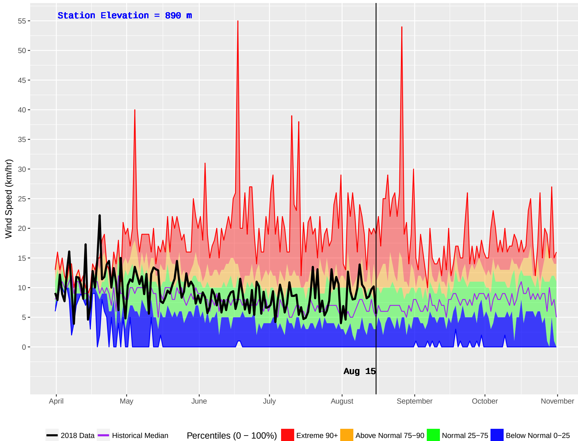
ISKUT (112) : Historical (1979–2016) and Current (2018) Daily Wind Speed
