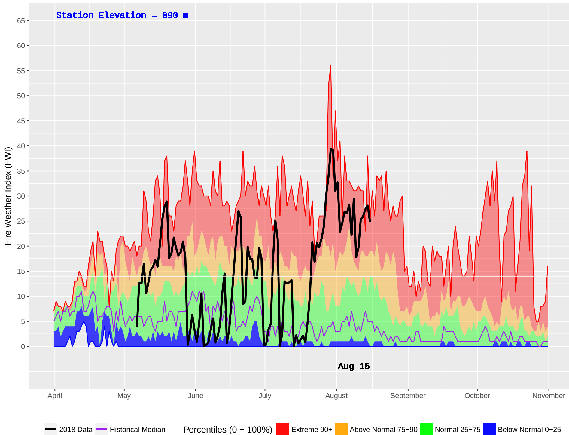
ISKUT (112) : Historical (1979–2016) and Current (2018) Daily Fire Weather Index (FWI)
